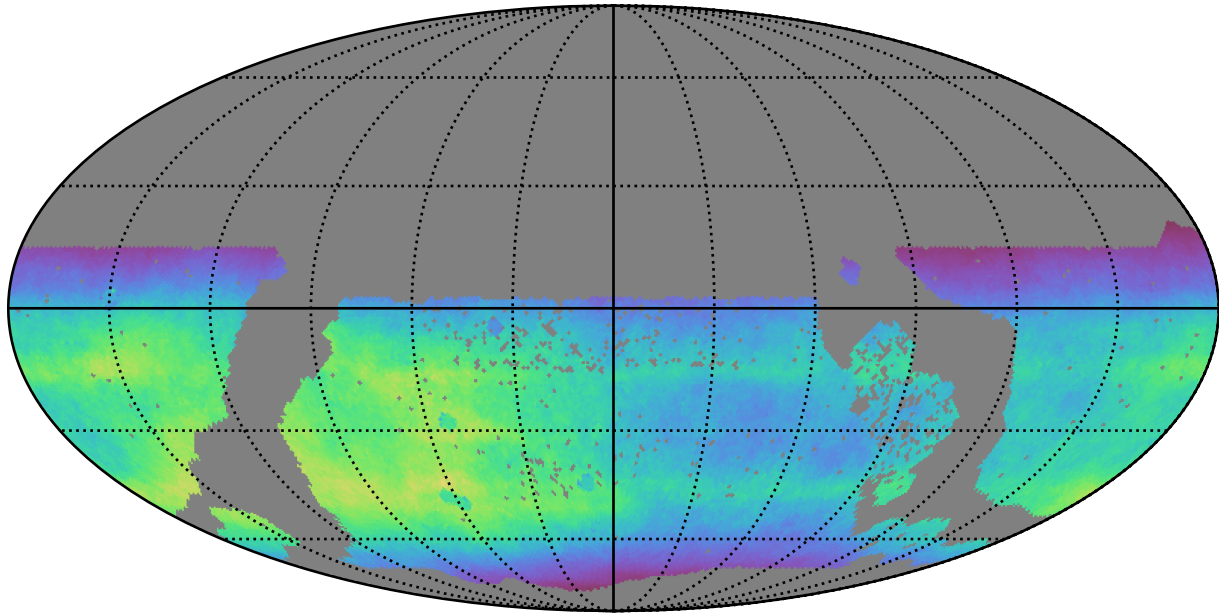
too_elab_r128_d3_gz_v3.4_10yrs WFD all bands: Normalized Teff
