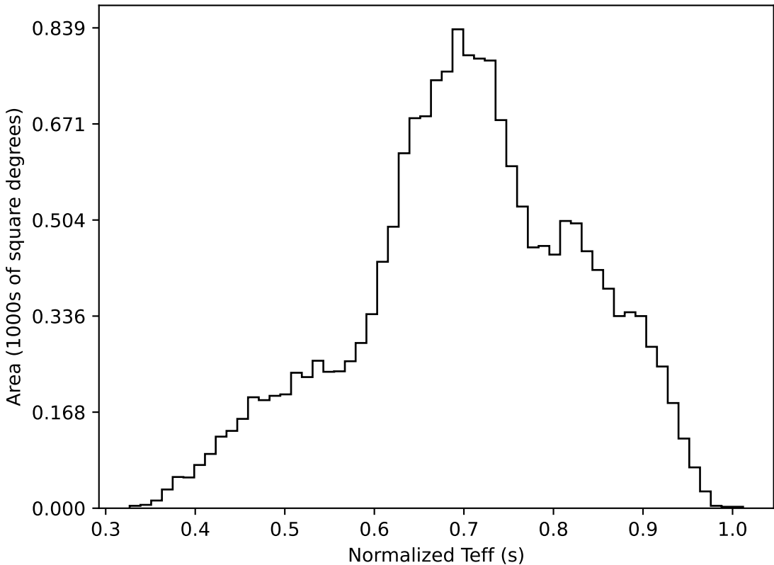
too_elab_r128_d3_gz_v3.4_10yrs WFD all bands: Normalized Teff
