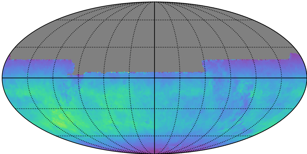
too_elab_r128_d3_gz_v3.4_10yrs All sky y band: Normalized Teff
