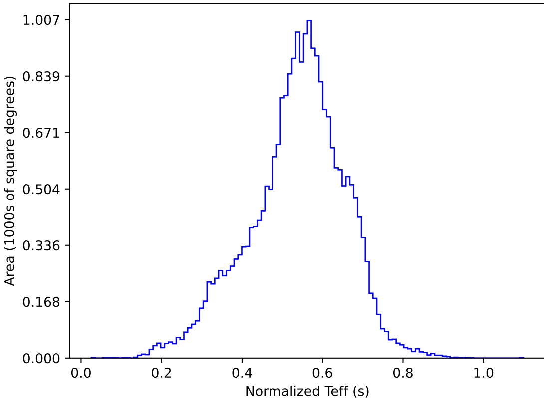
too_elab_r128_d3_gz_v3.4_10yrs All sky y band: Normalized Teff
