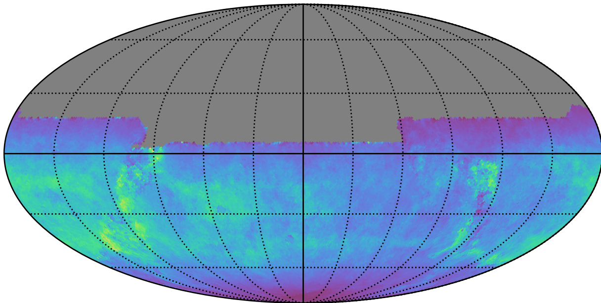
too_elab_r128_d3_gz_v3.4_10yrs All sky u band: Normalized Teff
