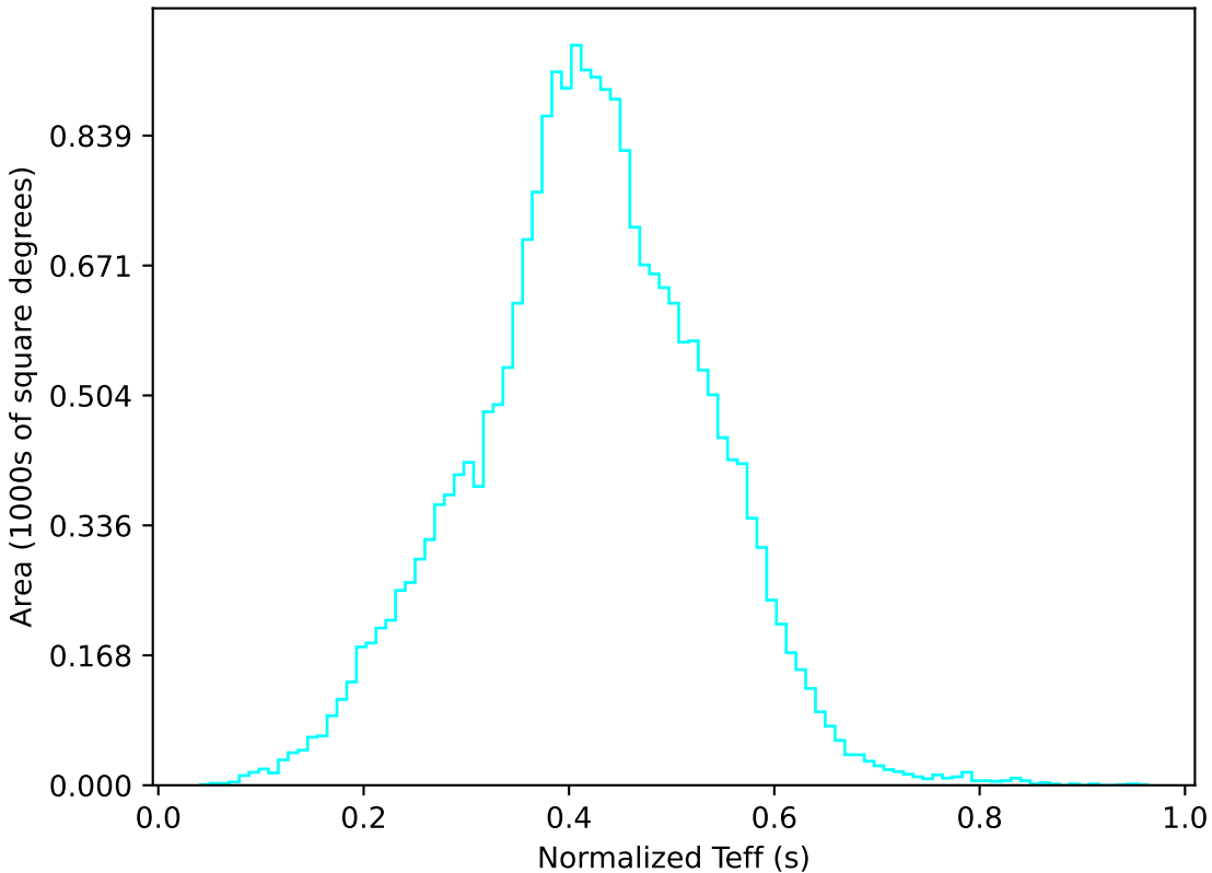
too_elab_r128_d3_gz_v3.4_10yrs All sky u band: Normalized Teff
