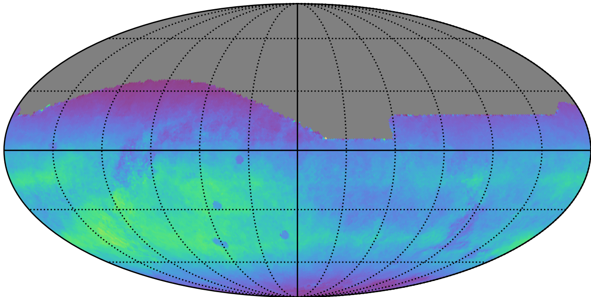
too_elab_r128_d3_gz_v3.4_10yrs All sky r band: Normalized Teff
