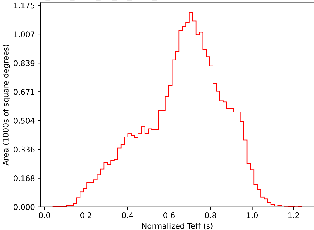
too_elab_r128_d3_gz_v3.4_10yrs All sky i band: Normalized Teff
