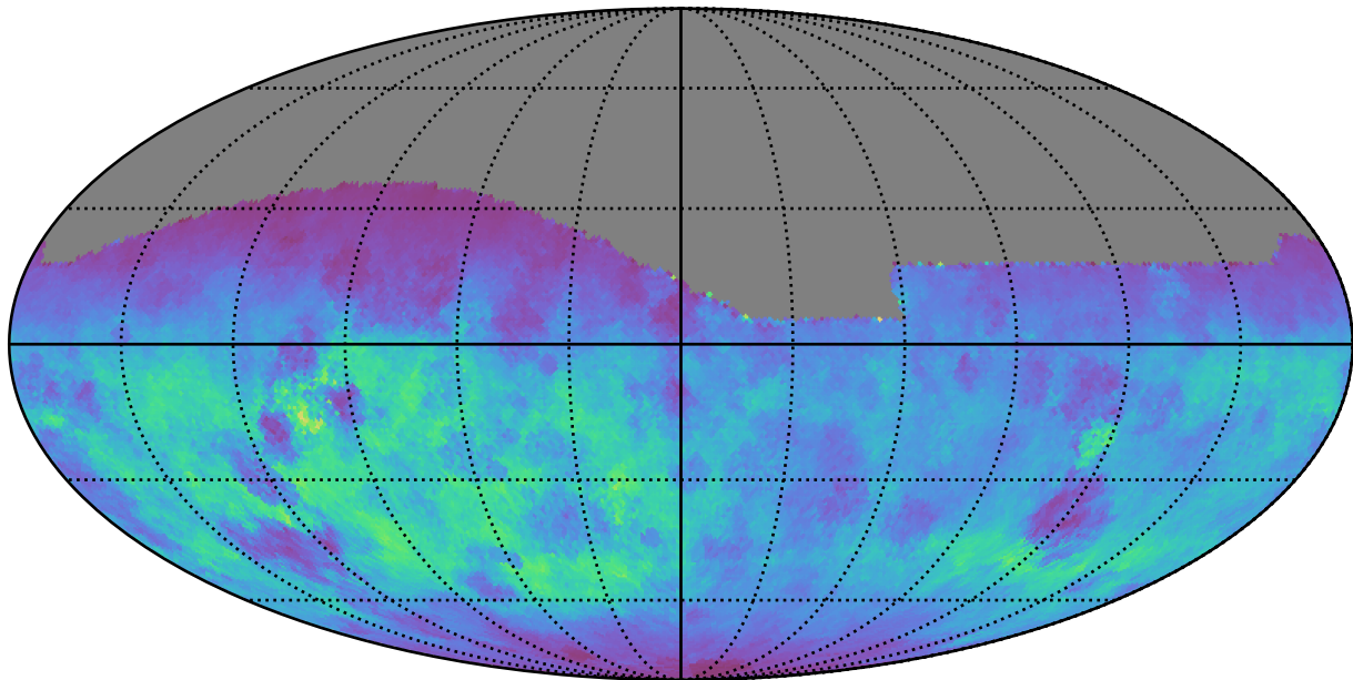
too_elab_r128_d3_gz_v3.4_10yrs All sky g band: Normalized Teff
