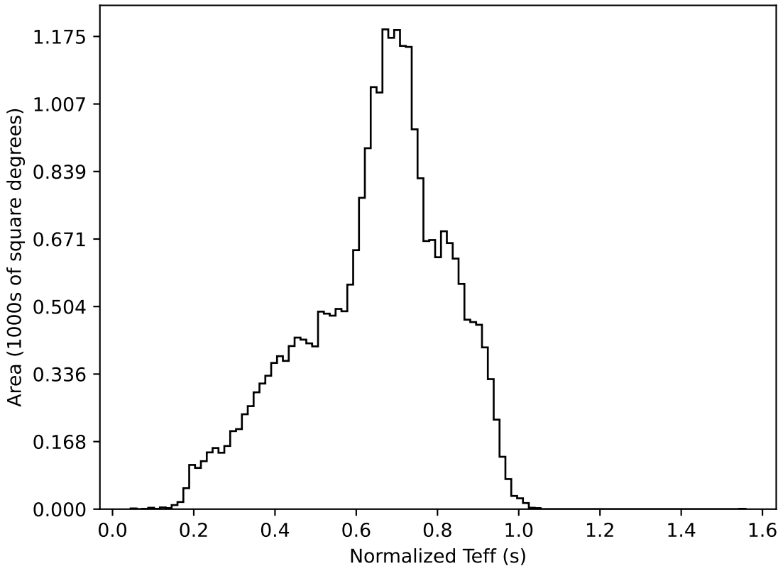
too_elab_r128_d3_gz_v3.4_10yrs All sky all bands: Normalized Teff
