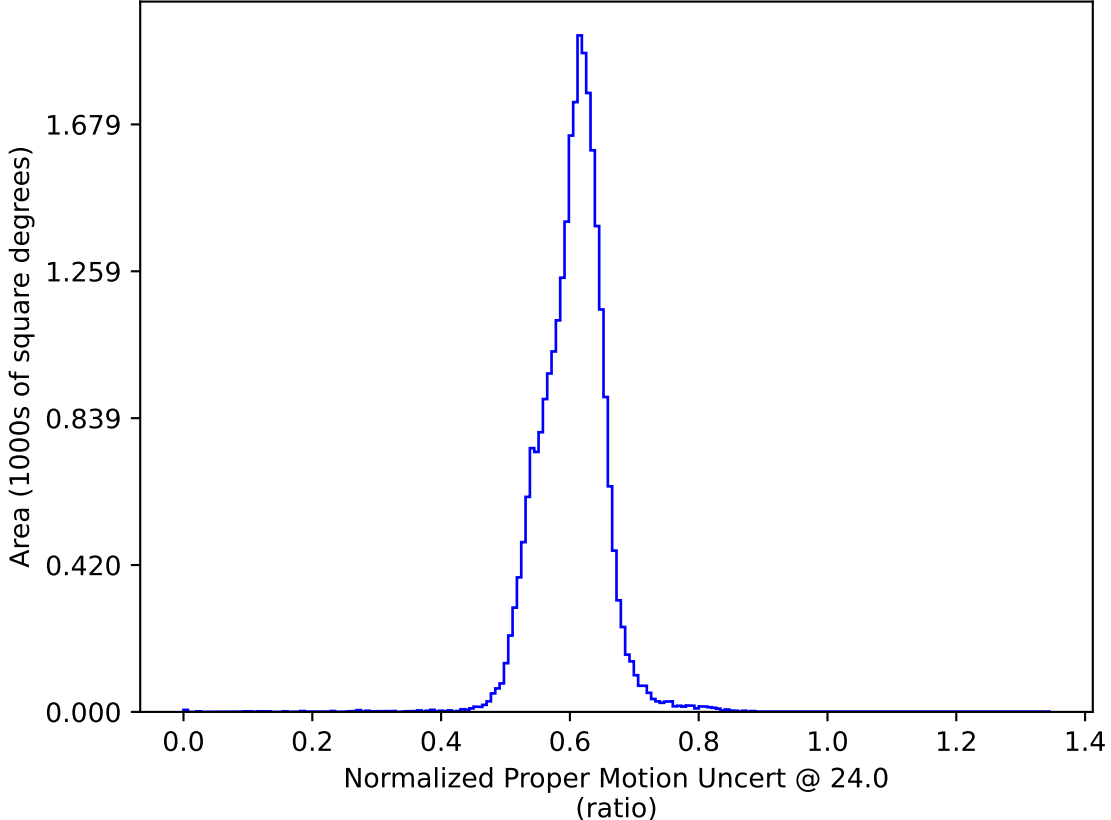
too_elab_r128_d3_gz_v3.4_10yrs All sky: Normalized Proper Motion Uncert @ 24.0
