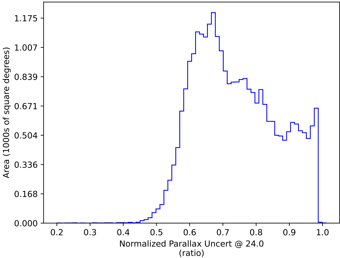
too_elab_r128_d3_gz_v3.4_10yrs All sky: Normalized Parallax Uncert @ 24.0
