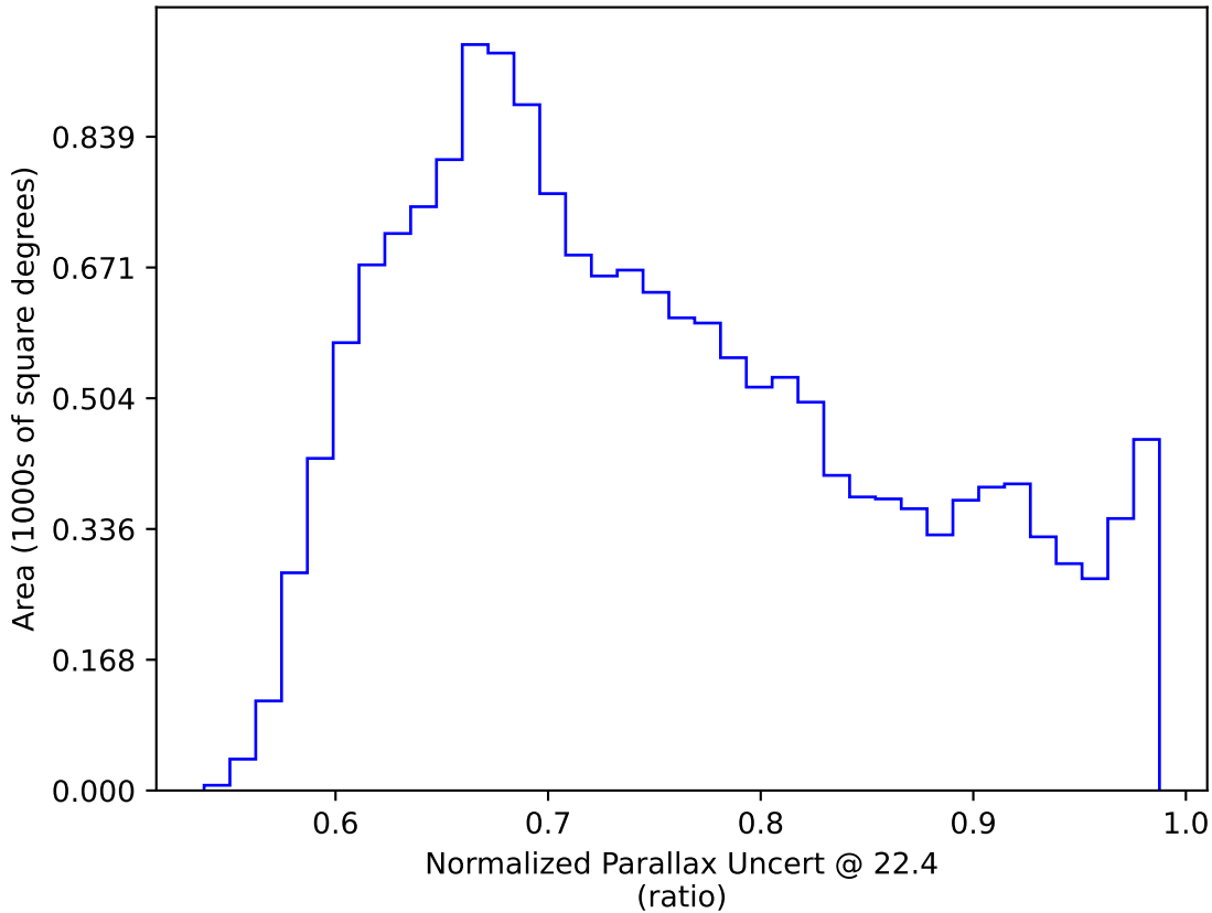
too_elab_r128_d3_gz_v3.4_10yrs WFD: Normalized Parallax Uncert @ 22.4
