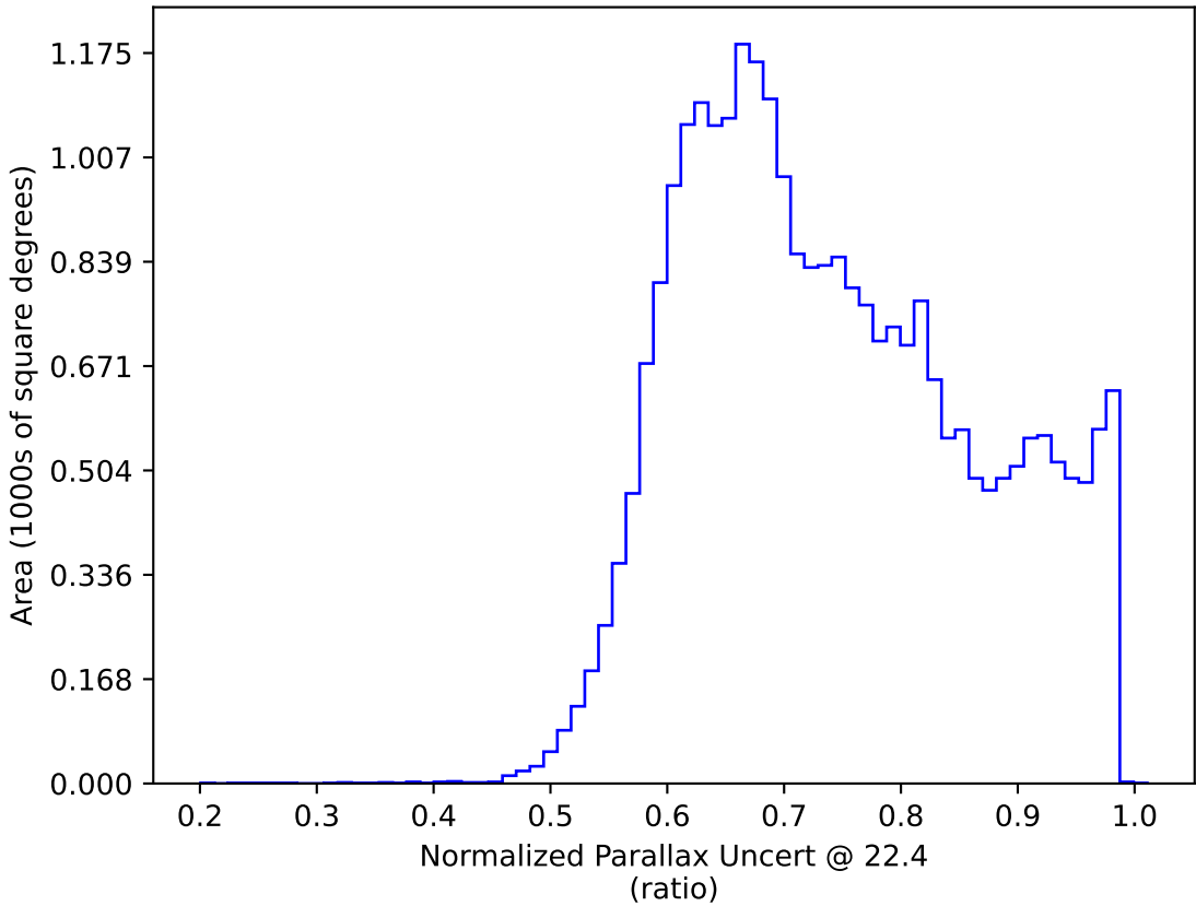
too_elab_r128_d3_gz_v3.4_10yrs All sky: Normalized Parallax Uncert @ 22.4
