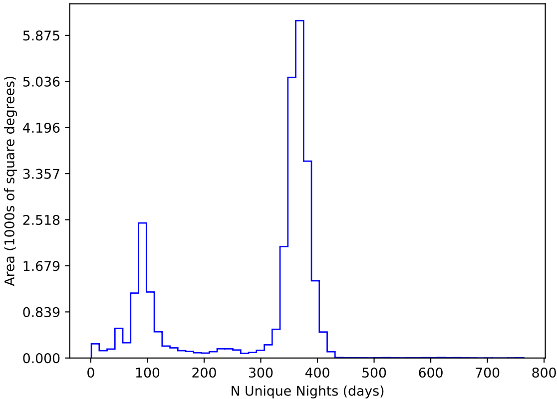
too_elab_r128_d3_gz_v3.4_10yrs All sky all bands: N Unique Nights
