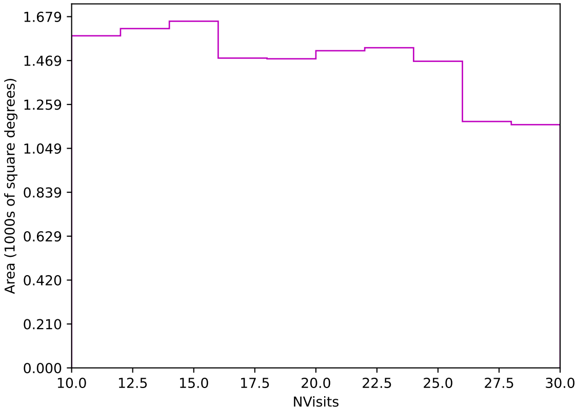
too_elab_r128_d3_gz_v3.4_10yrs Yr 3-4 z band: NVisits
