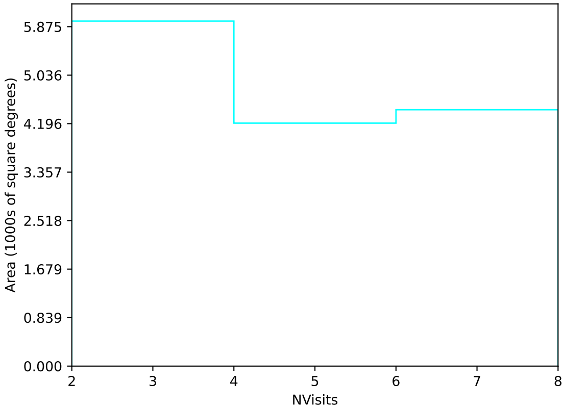
too_elab_r128_d3_gz_v3.4_10yrs Yr 3-4 u band: NVisits
