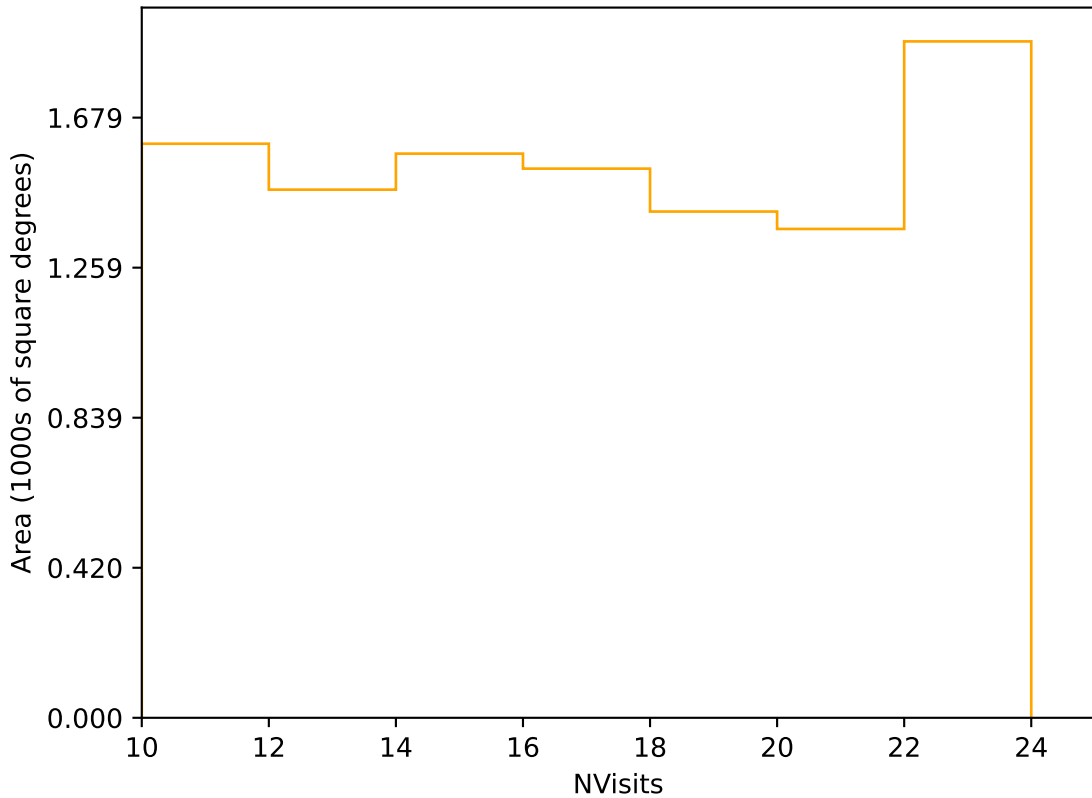
too_elab_r128_d3_gz_v3.4_10yrs Yr 3-4 r band: NVisits
