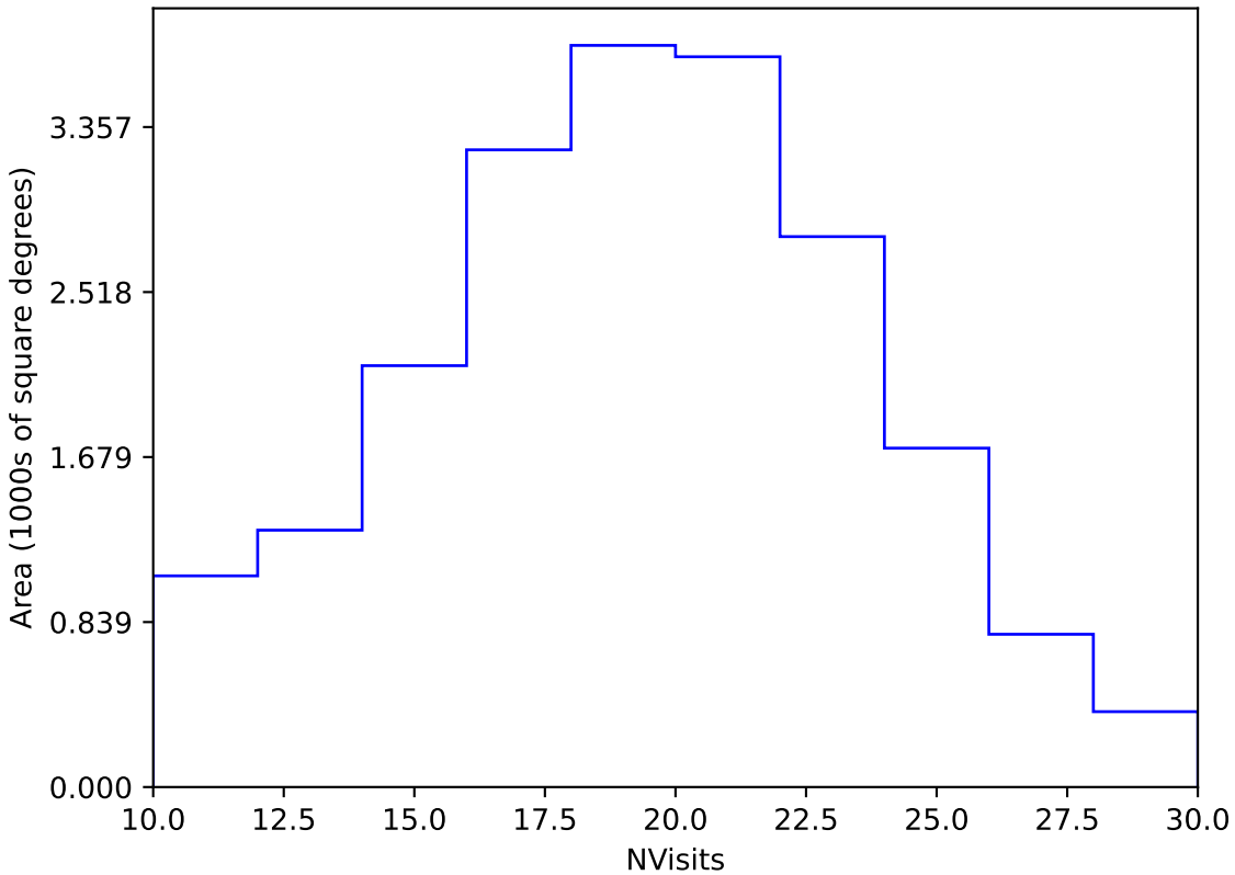
too_elab_r128_d3_gz_v3.4_10yrs Yr 1 y band: NVisits
