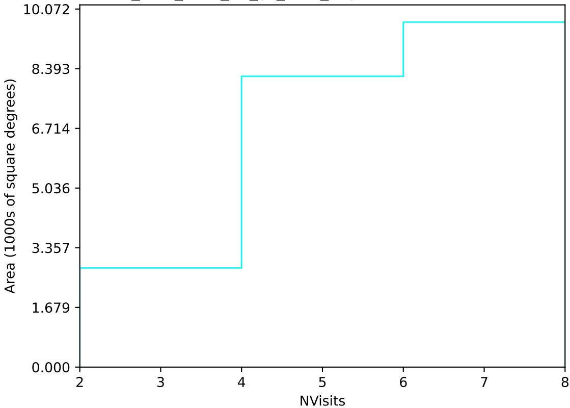
too_elab_r128_d3_gz_v3.4_10yrs Yr 1 u band: NVisits
