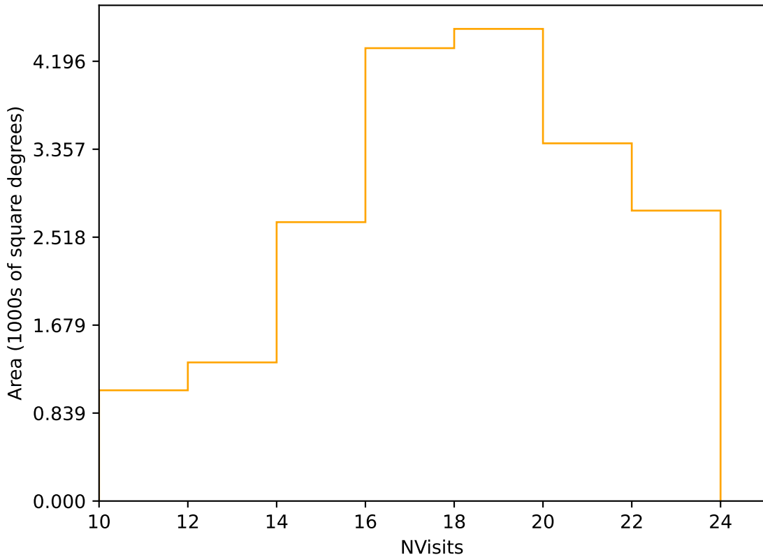
too_elab_r128_d3_gz_v3.4_10yrs Yr 1 r band: NVisits
