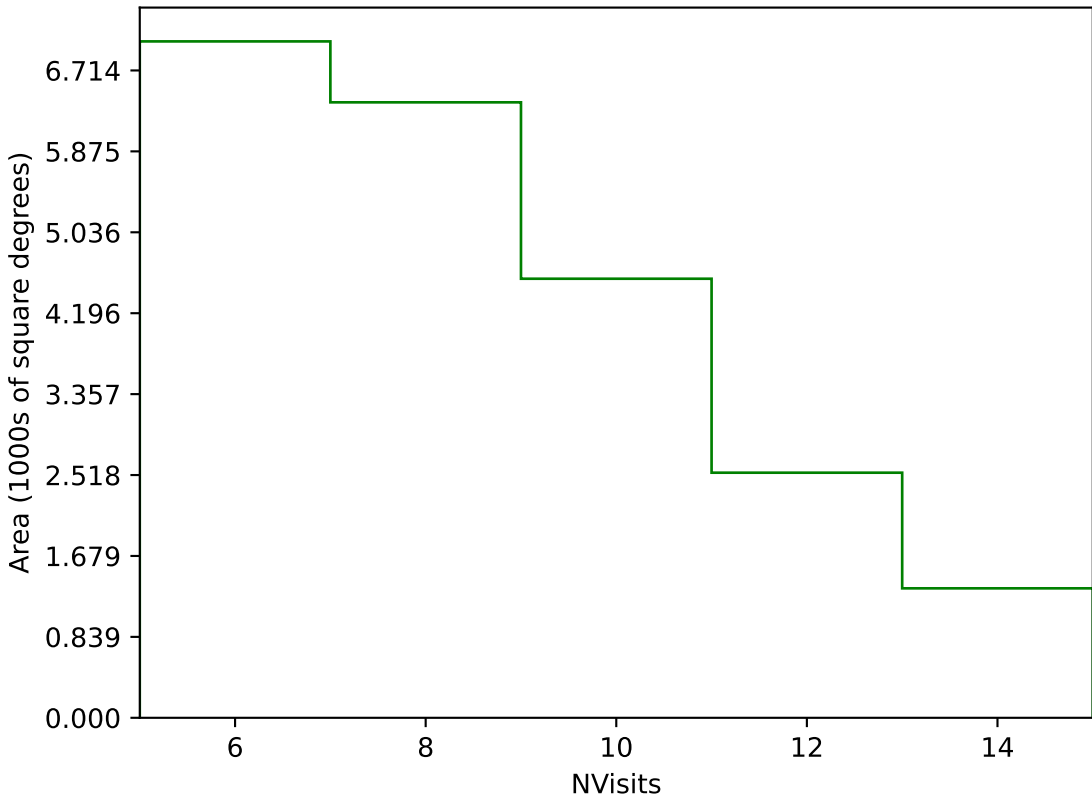
too_elab_r128_d3_gz_v3.4_10yrs Yr 1 g band: NVisits
