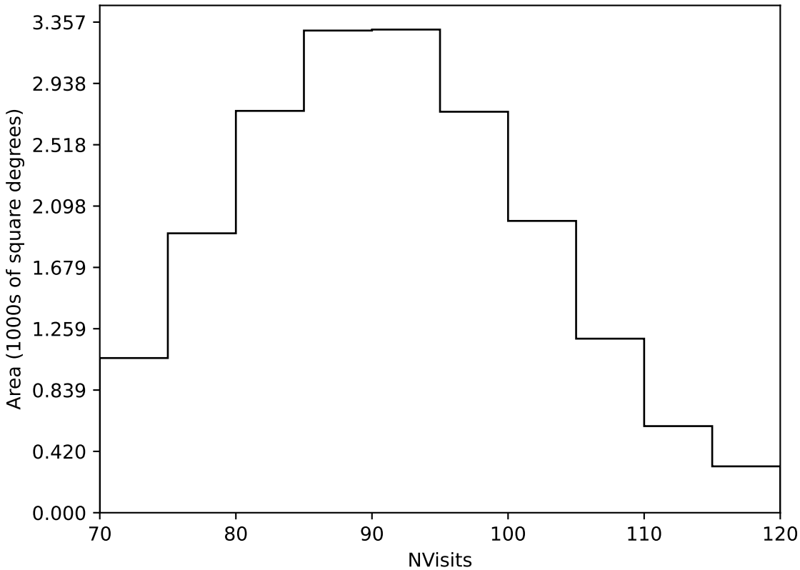
too_elab_r128_d3_gz_v3.4_10yrs Yr 1 all bands: NVisits
