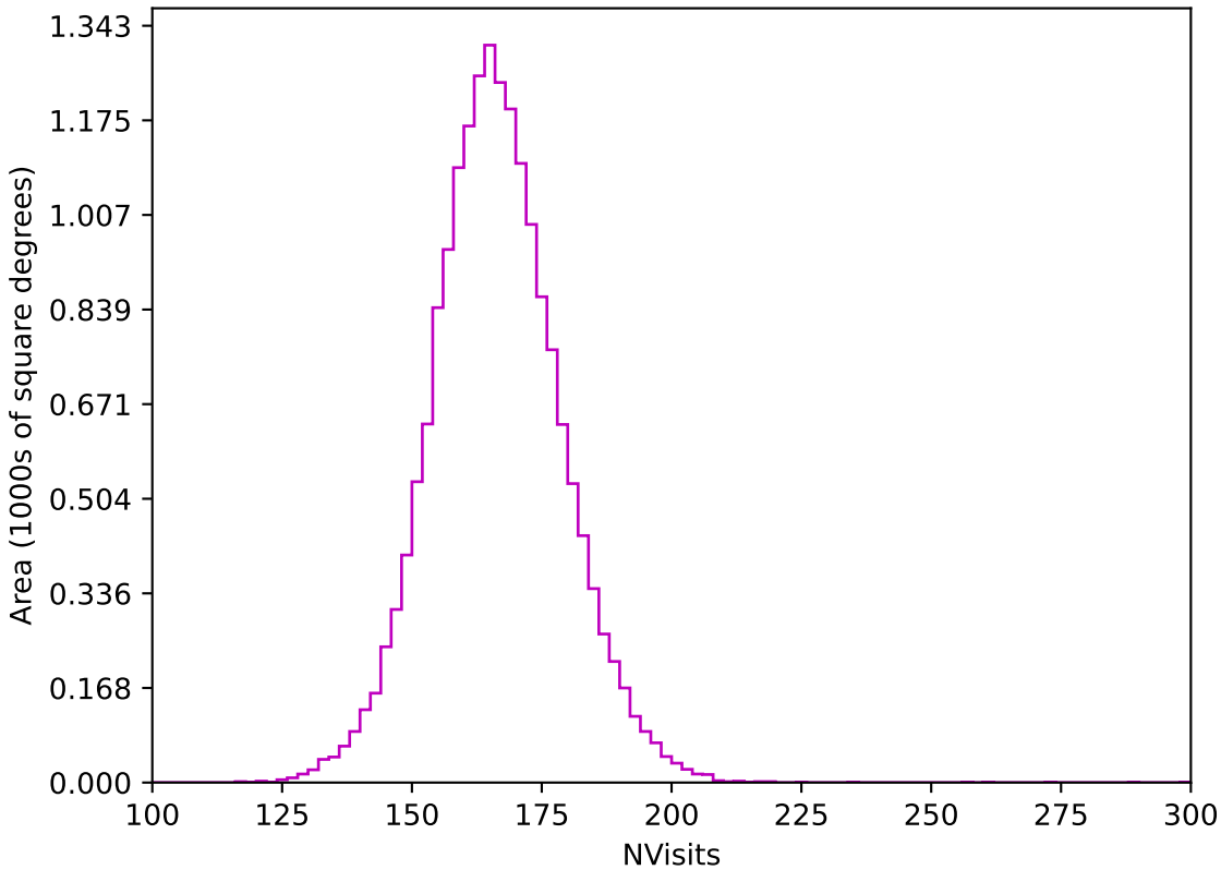
too_elab_r128_d3_gz_v3.4_10yrs WFD z band: NVisits
