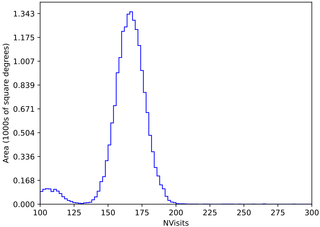
too_elab_r128_d3_gz_v3.4_10yrs WFD y band: NVisits
