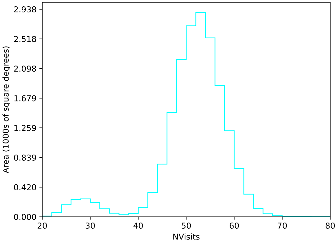
too_elab_r128_d3_gz_v3.4_10yrs WFD u band: NVisits
