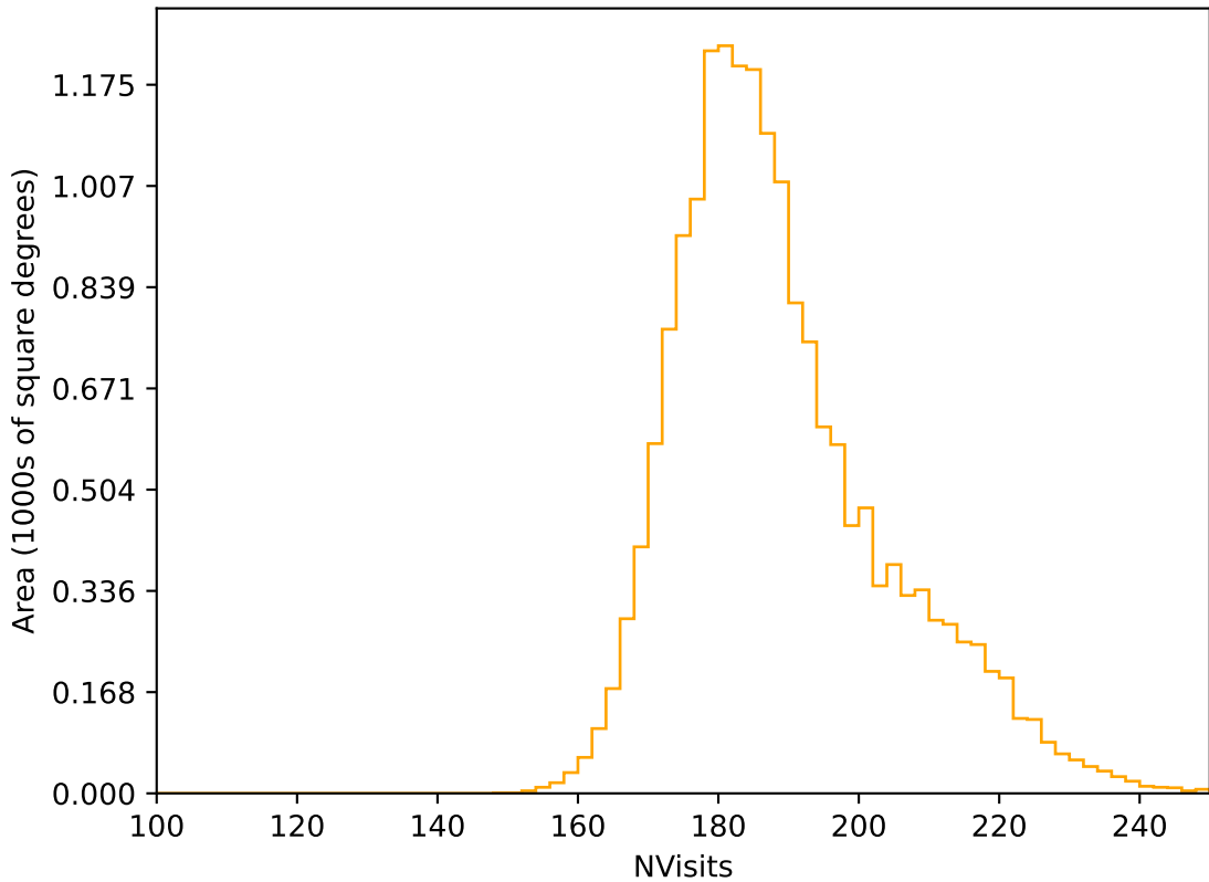
too_elab_r128_d3_gz_v3.4_10yrs WFD r band: NVisits
