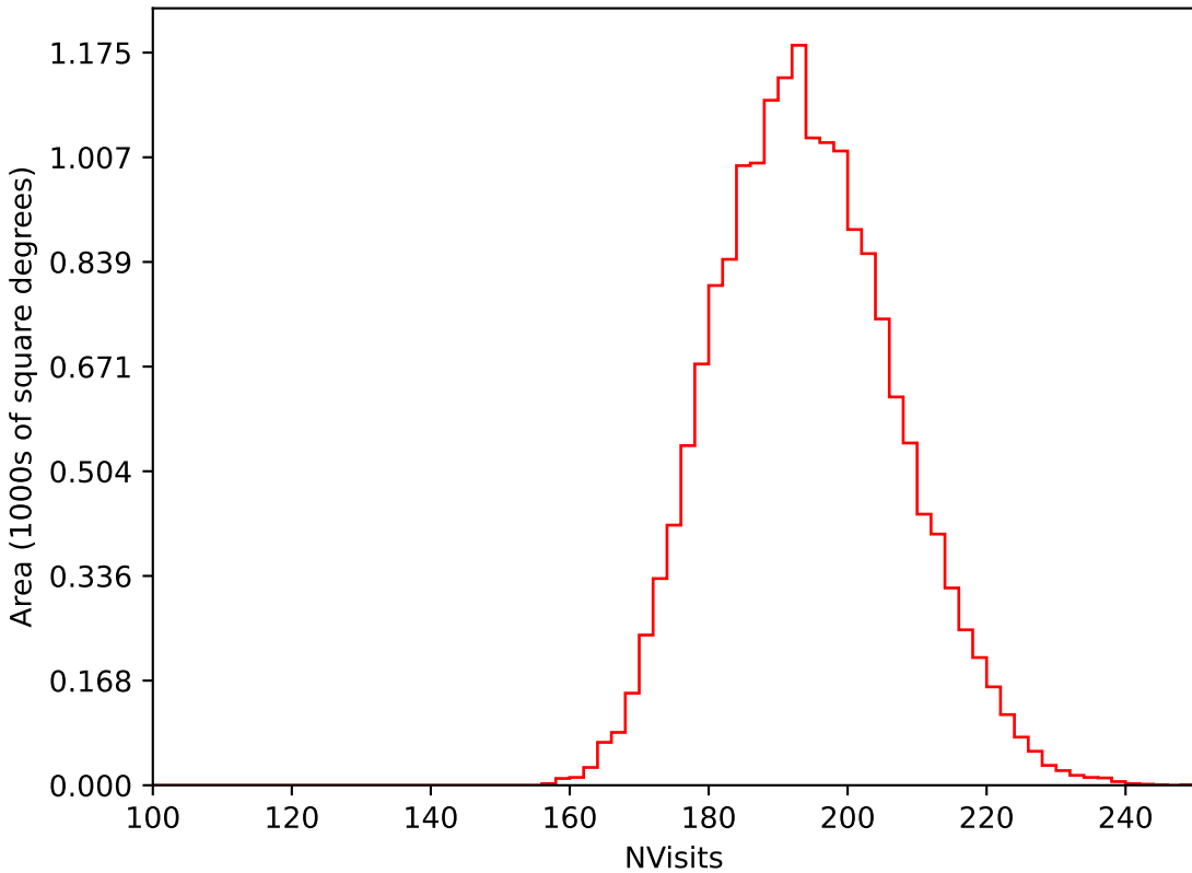
too_elab_r128_d3_gz_v3.4_10yrs WFD i band: NVisits
