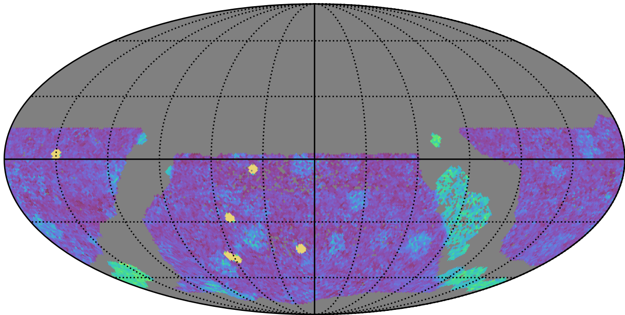
too_elab_r128_d3_gz_v3.4_10yrs WFD g band: NVisits
