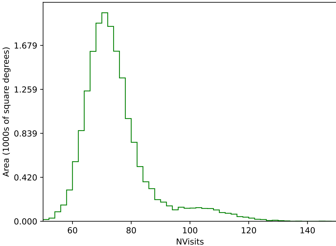
too_elab_r128_d3_gz_v3.4_10yrs WFD g band: NVisits
