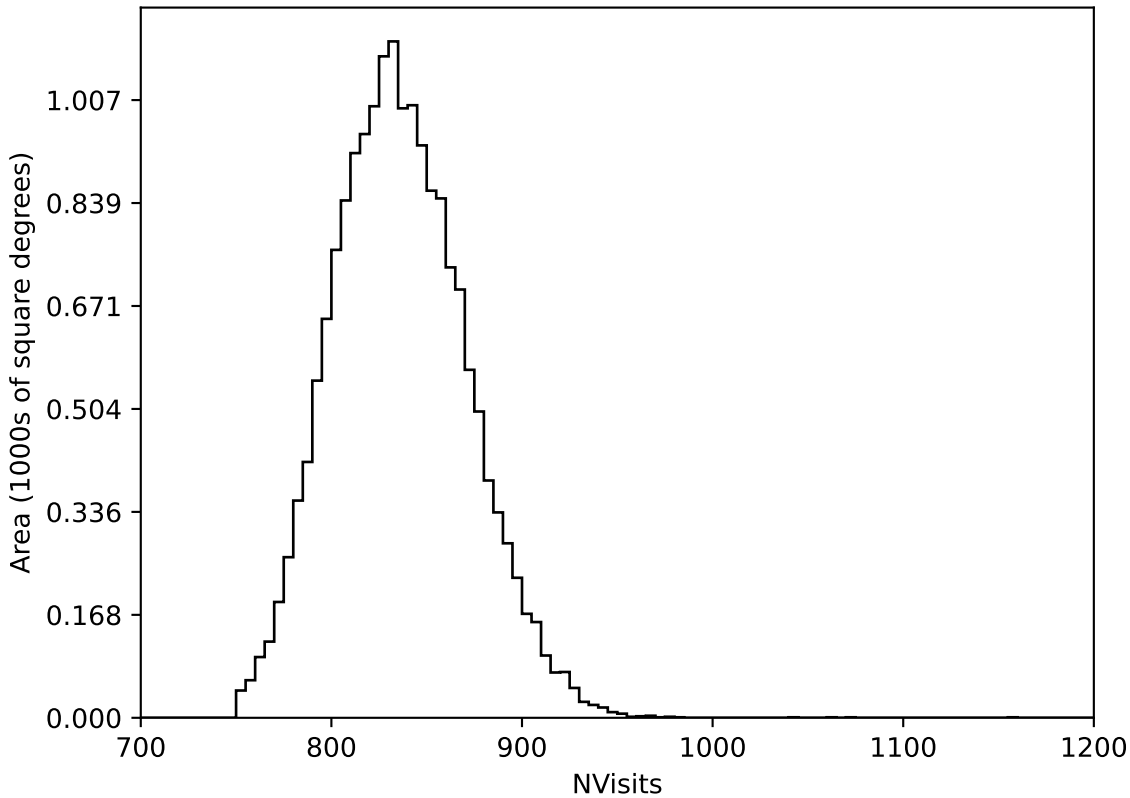
too_elab_r128_d3_gz_v3.4_10yrs WFD all bands: NVisits
