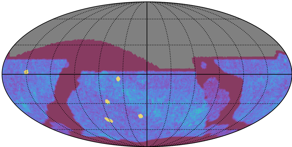
too_elab_r128_d3_gz_v3.4_10yrs All sky z band: NVisits
