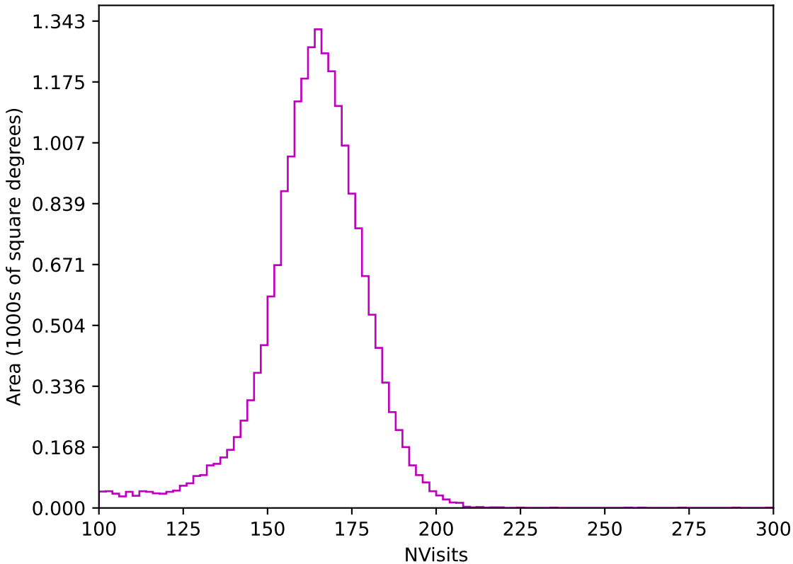
too_elab_r128_d3_gz_v3.4_10yrs All sky z band: NVisits
