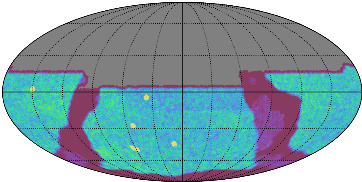
too_elab_r128_d3_gz_v3.4_10yrs All sky u band: NVisits
