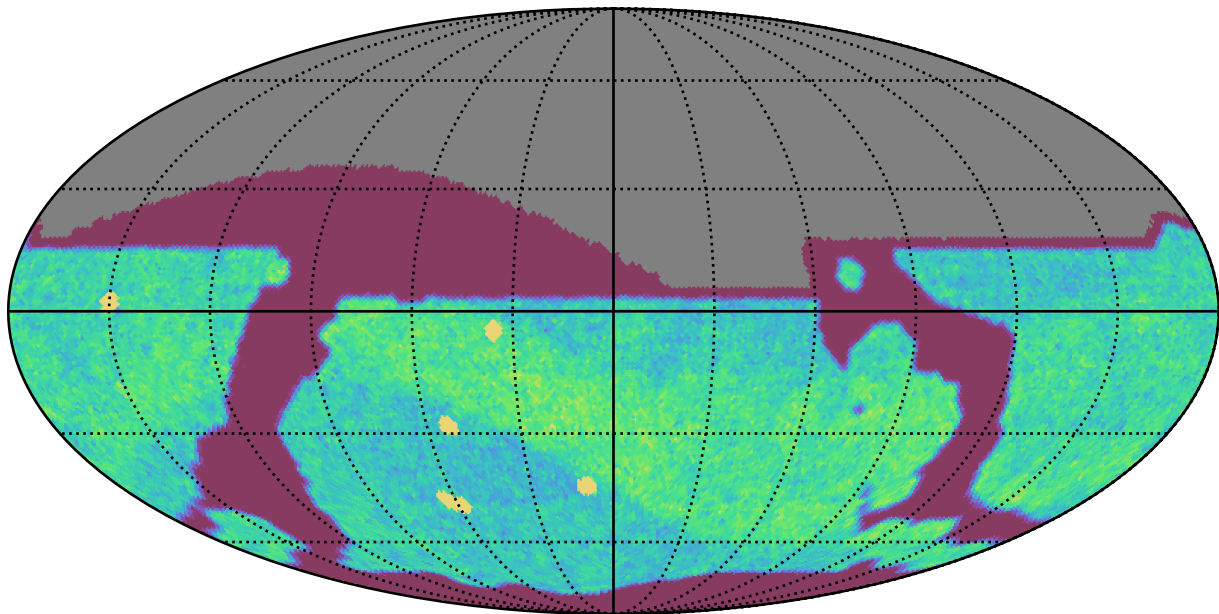
too_elab_r128_d3_gz_v3.4_10yrs All sky i band: NVisits
