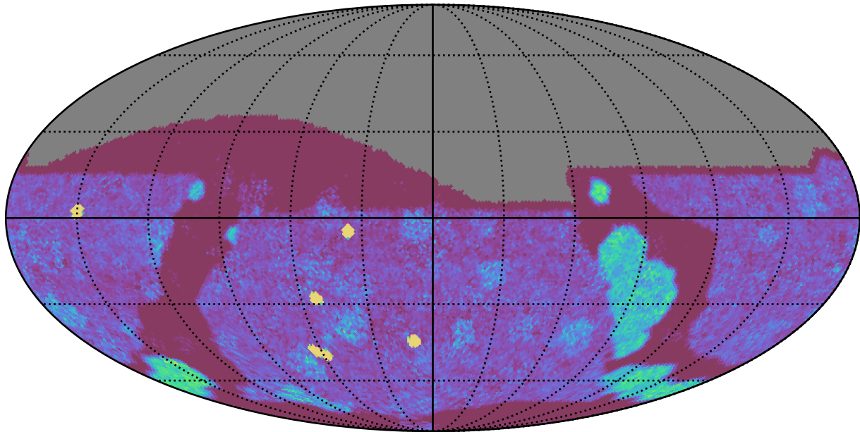
too_elab_r128_d3_gz_v3.4_10yrs All sky g band: NVisits
