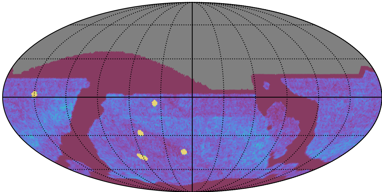
too_elab_r128_d3_gz_v3.4_10yrs All sky all bands: NVisits
