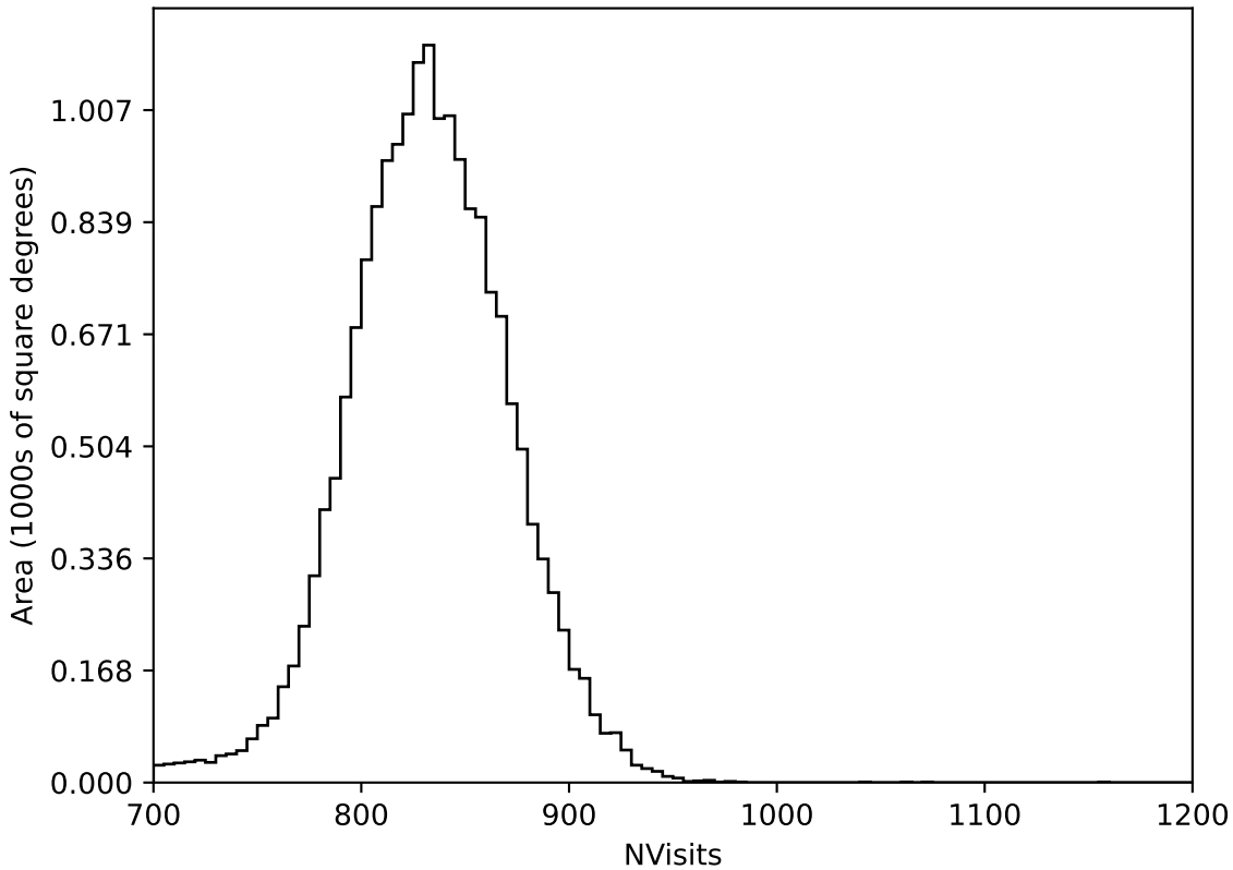
too_elab_r128_d3_gz_v3.4_10yrs All sky all bands: NVisits
