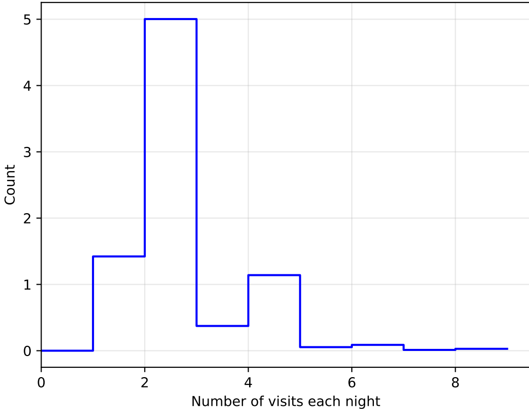
too_elab_r128_d3_gz_v3.4_10yrs WFD: NVisitsPerNight
