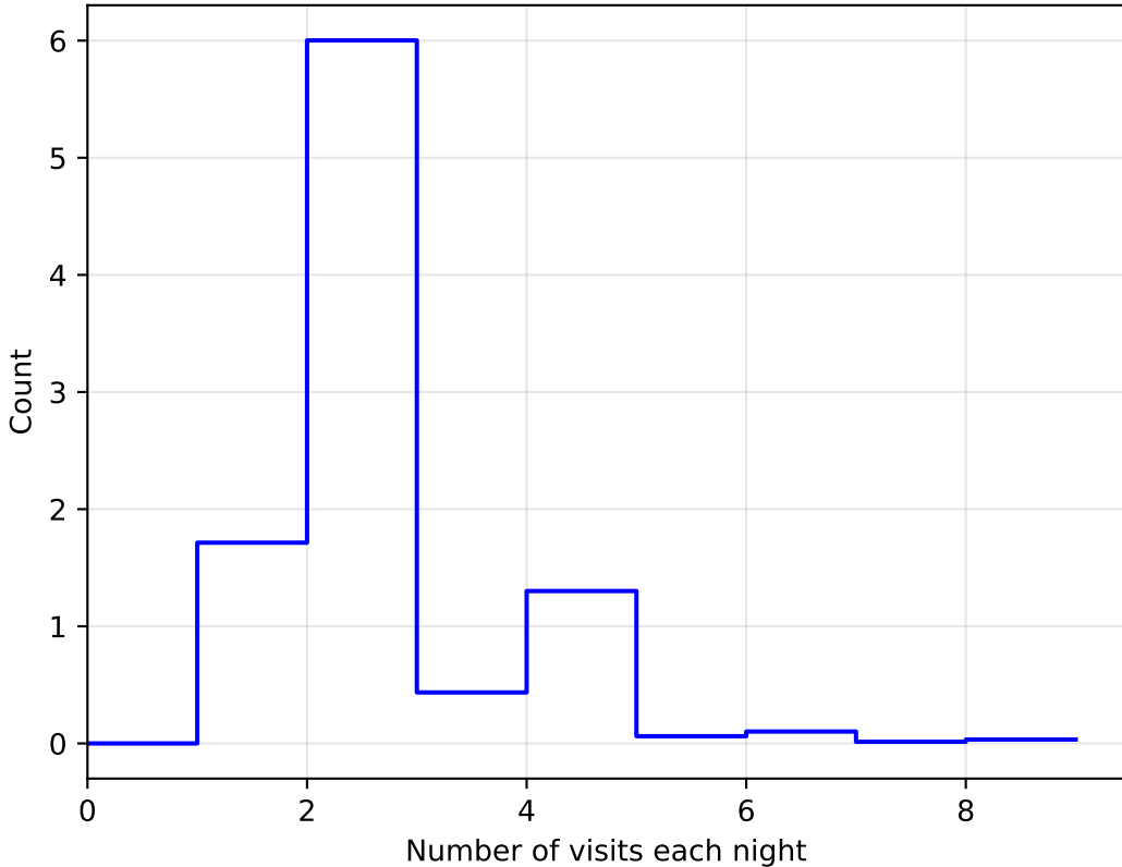
too_elab_r128_d3_gz_v3.4_10yrs All sky: NVisitsPerNight
