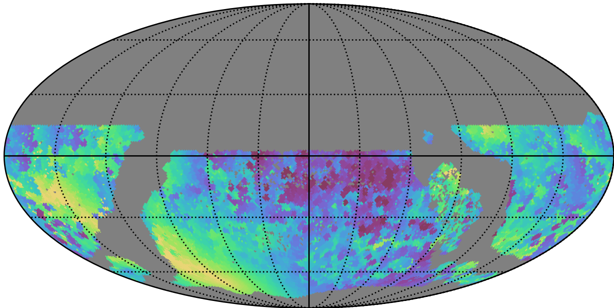
too_elab_r128_d3_gz_v3.4_10yrs WFD y band: Min solarElong
