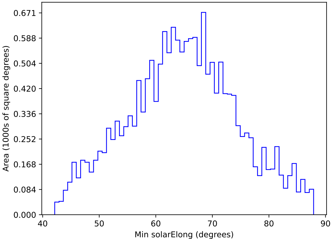
too_elab_r128_d3_gz_v3.4_10yrs WFD y band: Min solarElong
