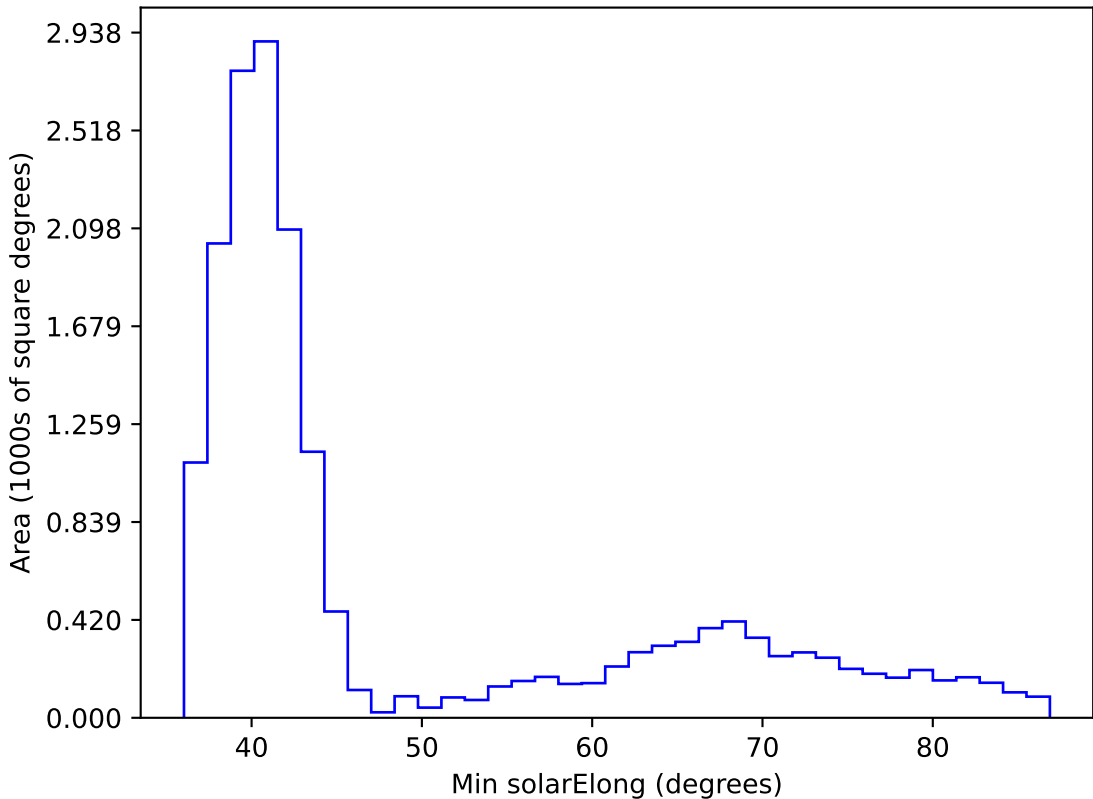
too_elab_r128_d3_gz_v3.4_10yrs WFD i band: Min solarElong
