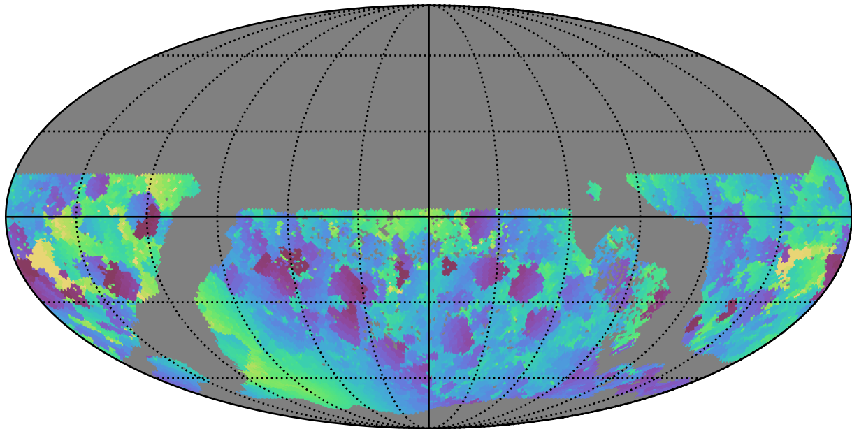
too_elab_r128_d3_gz_v3.4_10yrs WFD g band: Min solarElong
