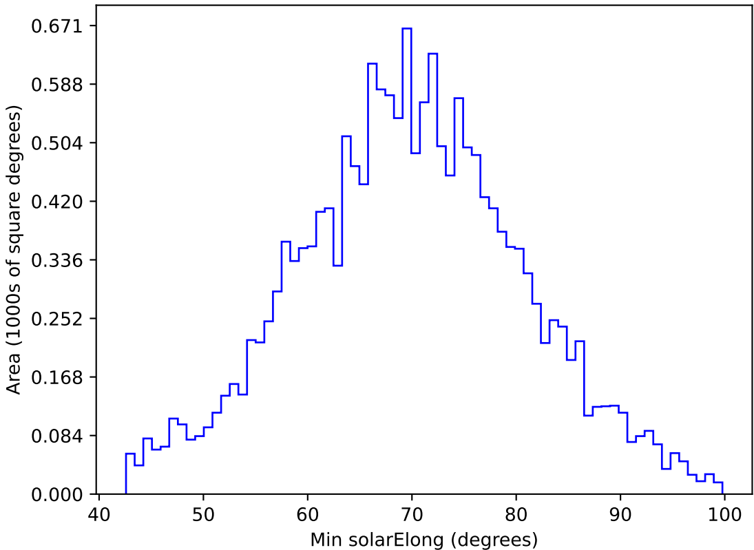
too_elab_r128_d3_gz_v3.4_10yrs WFD g band: Min solarElong
