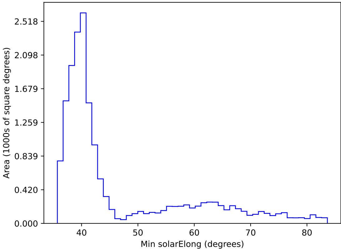
too_elab_r128_d3_gz_v3.4_10yrs WFD all bands: Min solarElong
