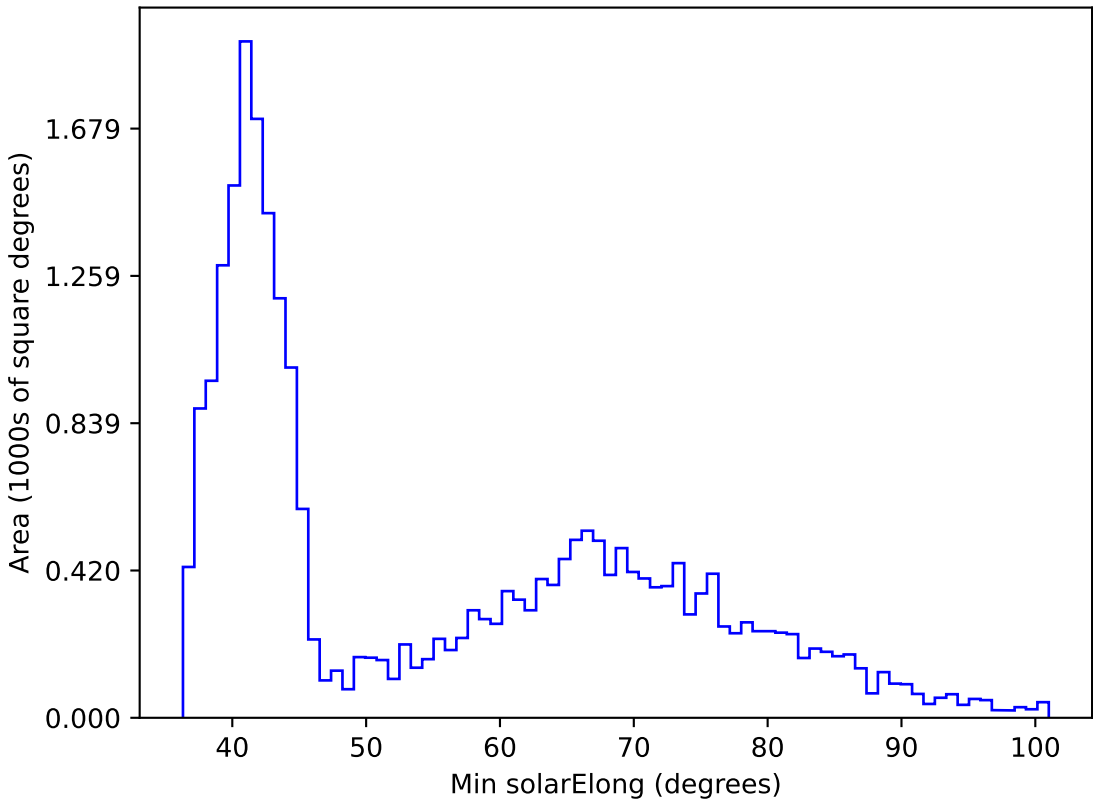
too_elab_r128_d3_gz_v3.4_10yrs All sky z band: Min solarElong
