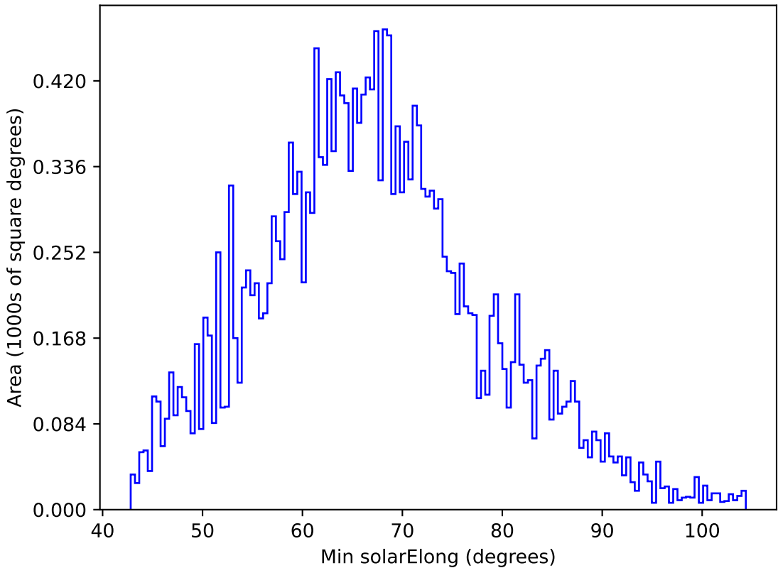
too_elab_r128_d3_gz_v3.4_10yrs All sky y band: Min solarElong
