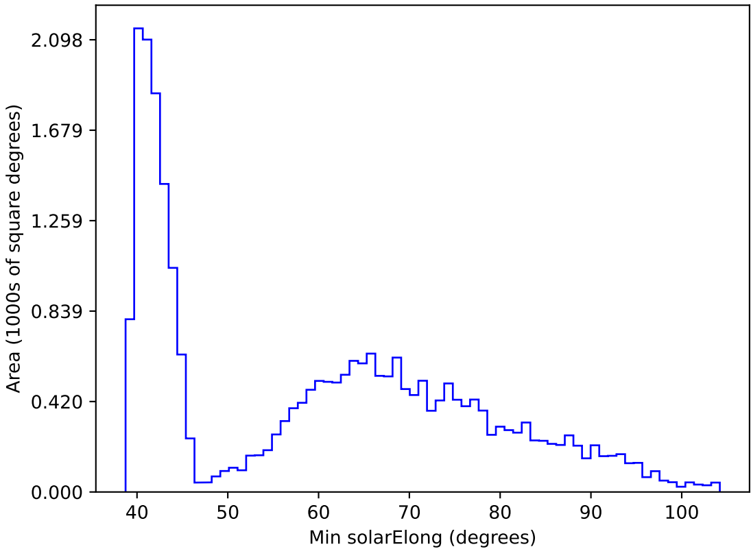
too_elab_r128_d3_gz_v3.4_10yrs All sky r band: Min solarElong
