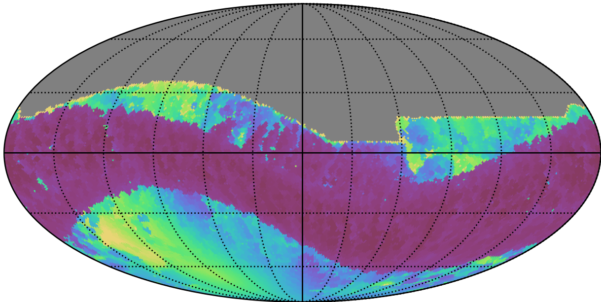
too_elab_r128_d3_gz_v3.4_10yrs All sky i band: Min solarElong
